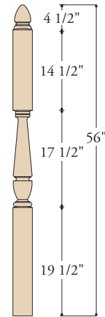
K-3046-ST 3-1/2" X 56" (F, T, O) LANDING
