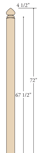
K-4006 3-1/2" X 72" LANDING
