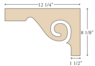
Tread Bracket K-8029 1/4" thick
