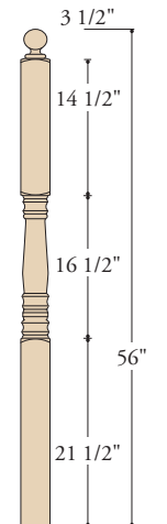
K-4505 3-1/2" X 56" (O) STARTING
