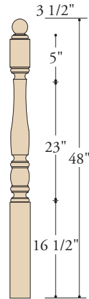
K-5548 3-1/2" X 48" (F, R, O) STARTING
