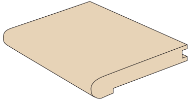
5-1/4" Landing Tread 32168-34-LTG for 3/4" floor 32168-12-LTG for 1/2" floor
