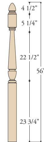
K-3042-ST 3-1/2" X 56" (F, T, O) STARTING/LANDING
