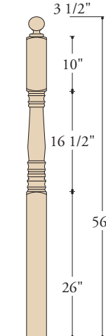
K-4503 3-1/2" X 56" (O) LANDING
