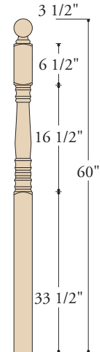
K-4304 3" X 60" STARTING/LANDING
