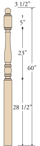
K-5560 3-1/2" X 60" (F, R, O) STARTING/LANDING
