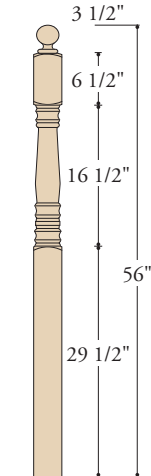
K-4504 3-1/2" X 56" (O) STARTING/LANDING
