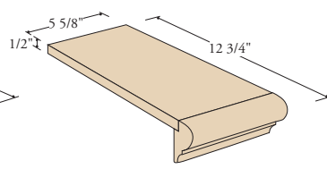
Tread Cap K-8072 5-5/8" x 11-1/2"
