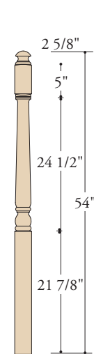
K-4042-A 3" X 54" (F) STARTING
