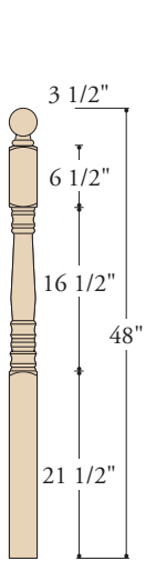
K-4300 3" X 48" STARTING
