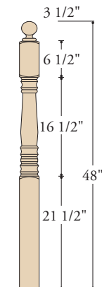
K-4500 3-1/2" X 48" (O) STARTING
