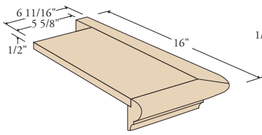
Tread Cap w/Mitered Return K-8071 5-5/8" x 11-1/2" Specify LH or RH (RH Shown)
