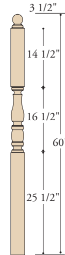
K-5546 3-1/2" X 60" (F, R, O) LANDING
