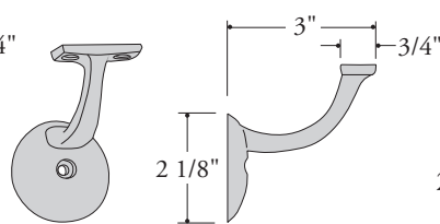
K-9802 Heavy Duty Wall Rail Bracket (Available in Matte Black, Oil Rubbed Bronze, Satin Black and Silver Vein Finish)
