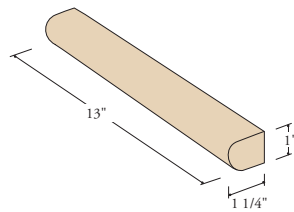
13" Return Nosing K-8080-13 1-1/4" x 1"
