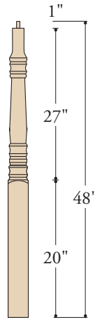
K-4271 3-1/2" X 48" (O) STARTING (Square Base)
