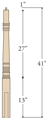
K-4272-RB 3-1/2" X 41" (O) VOLUTE (Round base, loose dowel)
