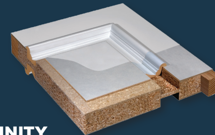
INFINITY Inlaid Moulding Doors
