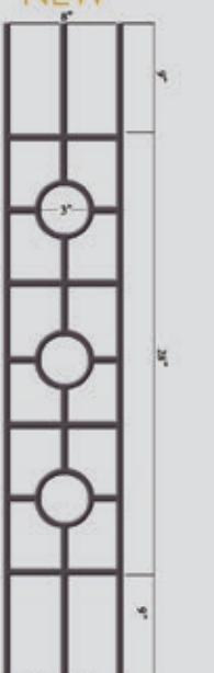
HF 9.4.44 Ends: 1/2" Sq. Height: 46" Wt. 4.9 lbs. TUBULAR (Rake)
