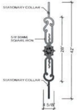
PIECE F FITS LEVEL BALCONY OR STRAIGHT RAIL
