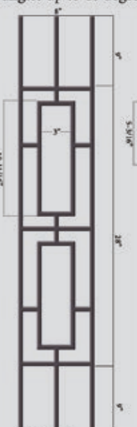
HF 9.4.22 Ends: 1/2" Sq. Height: 46" Wt. 4.7 lbs. TUBULAR (Rake)
